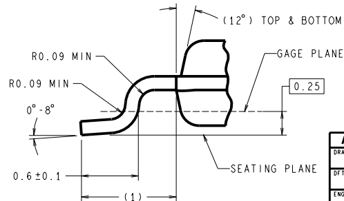
DETAIL A TYPICAL, SCALE: 40X
